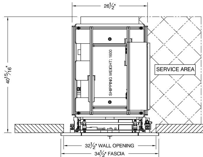
20X20X38 AUTOCLAVE SINGLE DOOR, RECESSED
