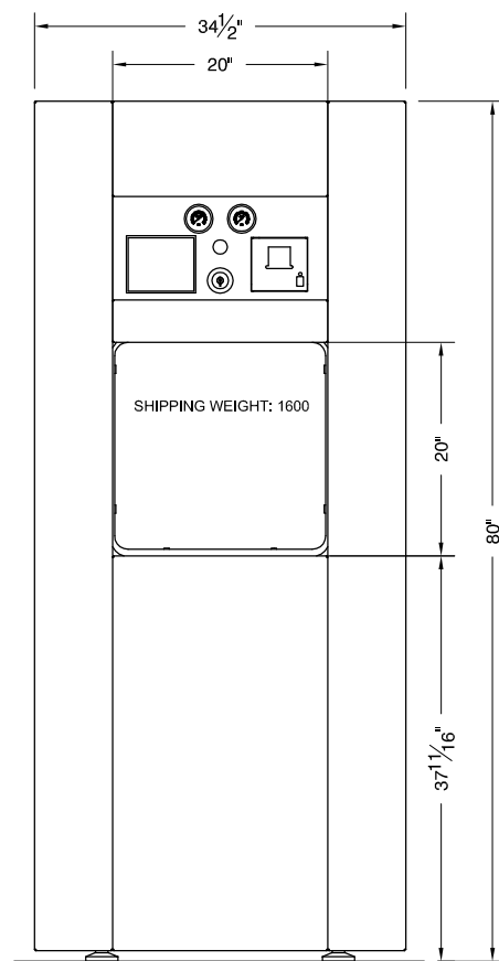
20X20X38 AUTOCLAVE SINGLE DOOR, FRONT VIEW
