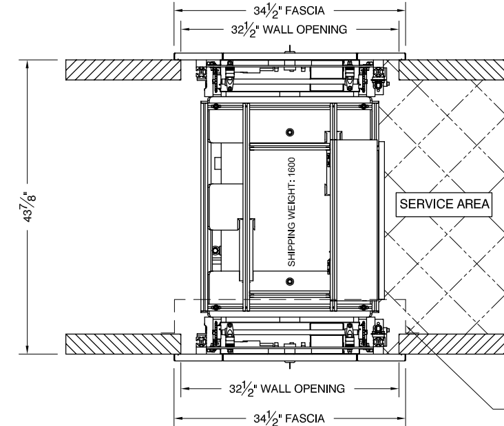
20X20X38 AUTOCLAVE DOUBLE DOOR, RECESSED
