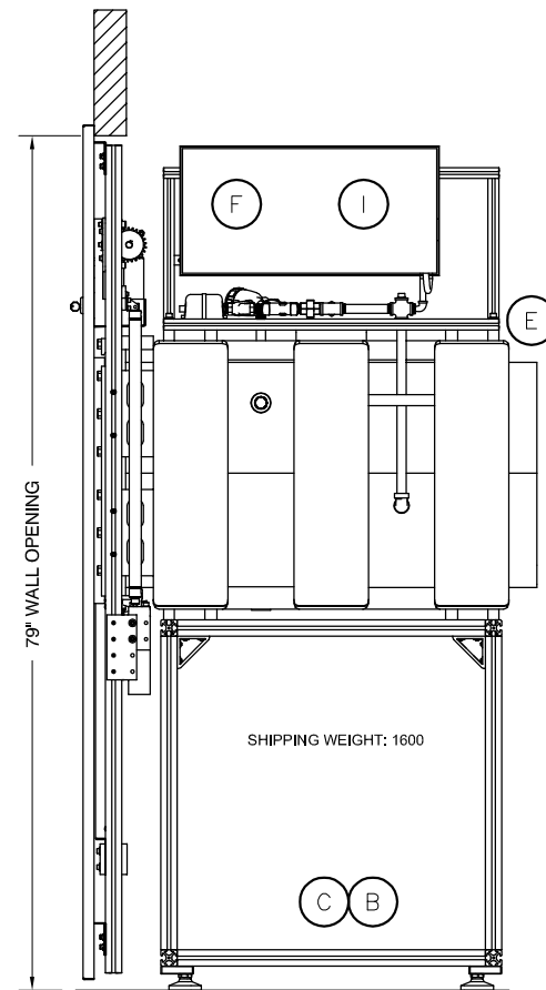
20X20X38 AUTOCLAVE SINGLE DOOR, SIDE VIEW
